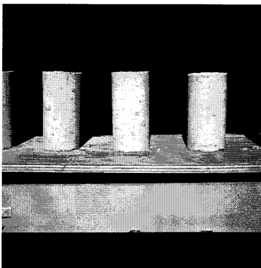
Fig. 12 Test blocks of rammed earth with various cacti embedded
