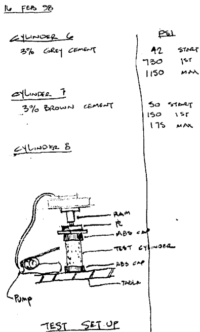
Fig.10 Student sketch of compression test
