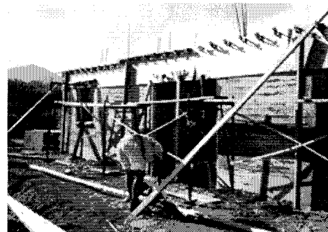
Fig. 8 Bond beam forms assembled at top of rammed earth walls
