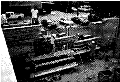
Fig.2 Forms staggered vertically as walls are tamped
