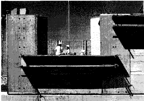
Fig.1 Plywood and pipe clamps form system devised for classroom facility
