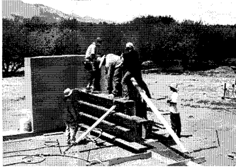
Fig. 6 Setting corner forms for Gila residence
