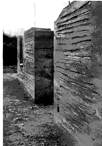
Fig. 7 Wall with embedded saguaro cactus ribs
